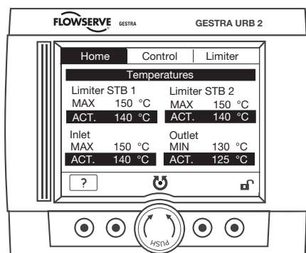
URB 2 Home screen (hot-water boiler)
