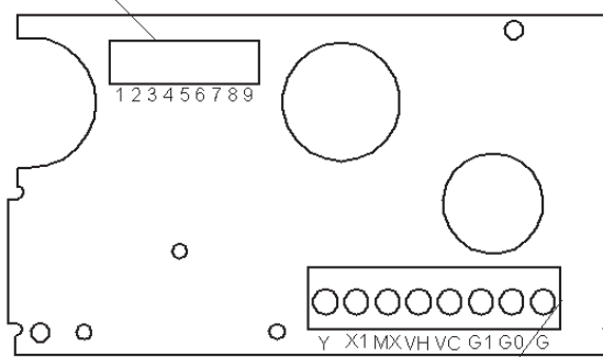
FIG. 1 TERMINAL BOARD
