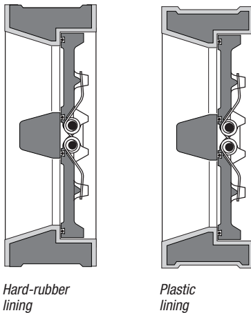
BB with lining from DN 150
